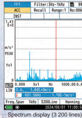
Spectrum display (3 200 lines)
