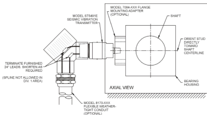
Figure 2: Flying leads spliced in conduit elbow.
