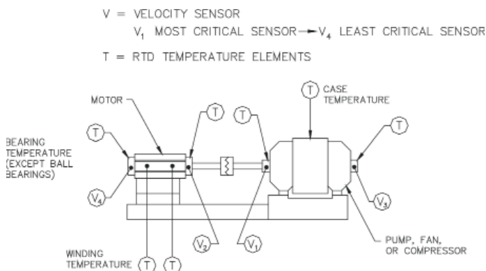
Figure 1: Horizontal mounting for casing vibration measurements.
