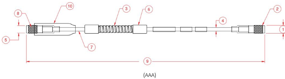
FIGURE 3: MX2031 Extension Cable
